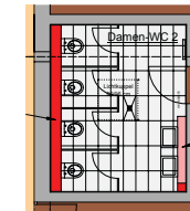
Detail Damen-WC M1.50
